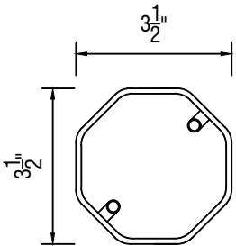
FRONT VIEW (OCTAGON RECEPTACLE BOX)
