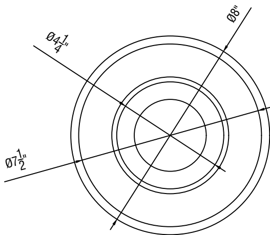
BOTTOM VIEW (LED LIGHT)
