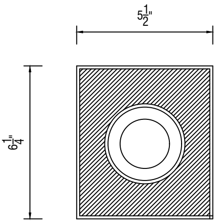
TOP VIEW (COVER PLATE )
