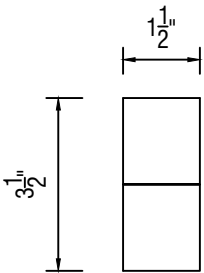
SIDE VIEW (OCTAGON RECEPTACLE BOX)
